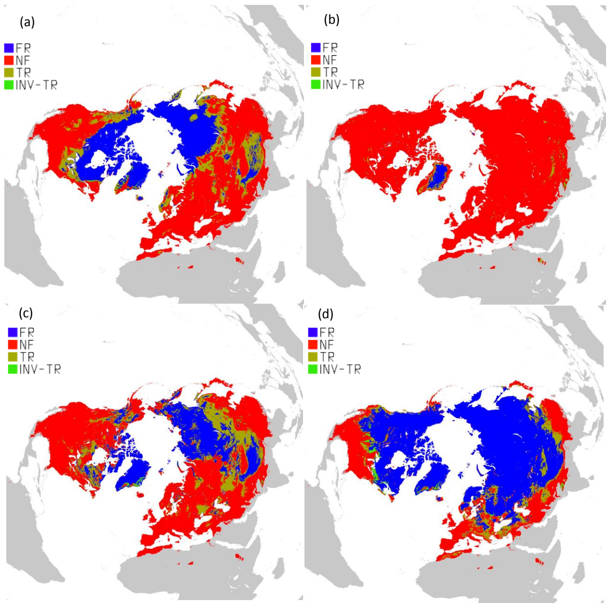
Figure 3: Selected daily combined (CO) FT-ESDR classification results for 2016, where: (a) DOY (Day of Year) =100, (b) DOY=200, (c) DOY=300, and (d) DOY=360; white and grey colors denote respective open water bodies and land areas outside of the FT-ESDR domain; FR (AM and PM frozen), NF (AM and PM thawed), TR (AM frozen and PM thawed) and INV-TR (AM thawed and PM frozen).
