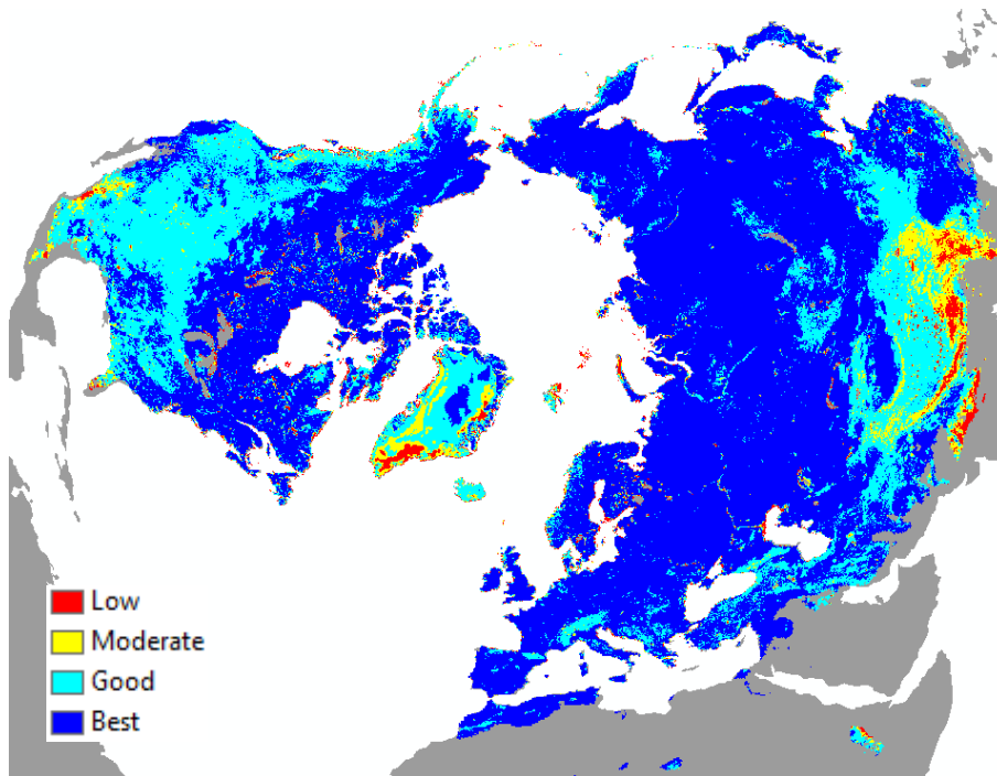
Figure 2: FT-ESDR annual quality assurance (QA) map for 2012, aggregated into low (estimated mean annual spatial classification agreement < 70%), moderate (70-80%), good (80-90%) and best (>90%) relative quality categories. Land areas outside of the FT-ESDR domain are denoted by grey shading.
