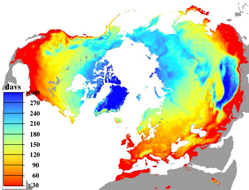
Figure 1: Mean annual frozen season (frozen or transitional status) over the 15-year (2002-2014) record and Polar FT-ESDR domain; white and grey colors denote respective open water bodies and land areas outside of the FT-ESDR domain.
